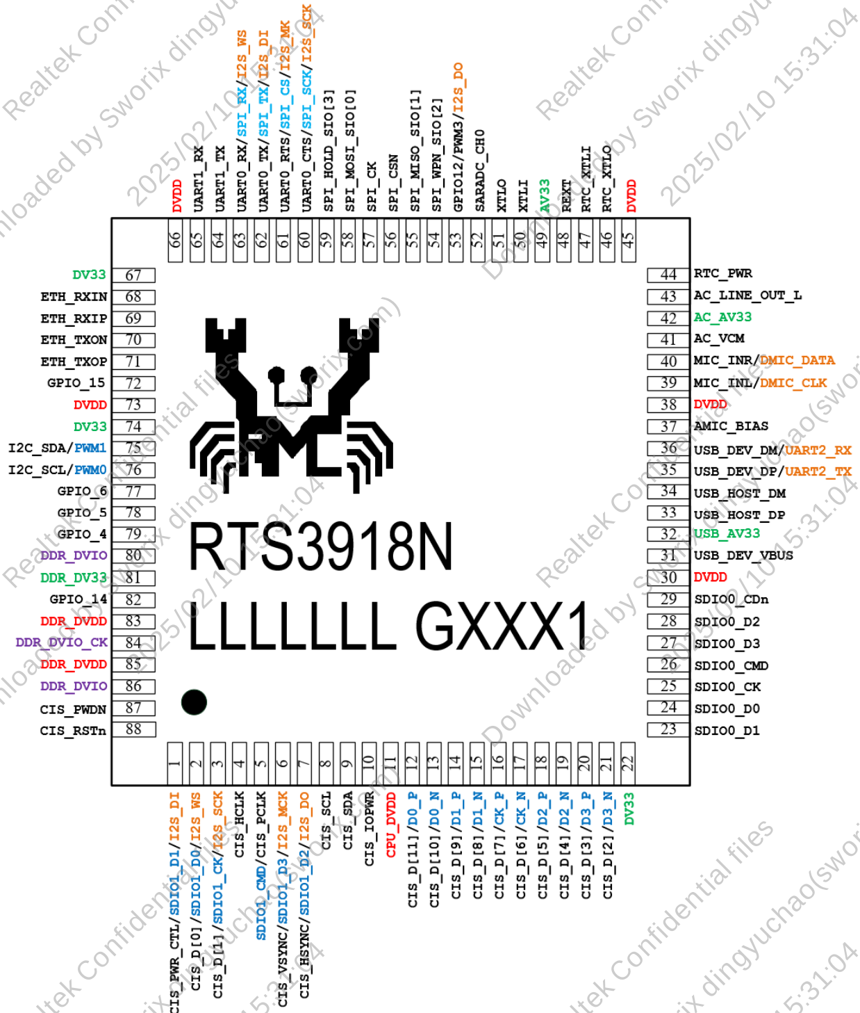
Figure 4-1 RTS3918N QFN88 pin define
