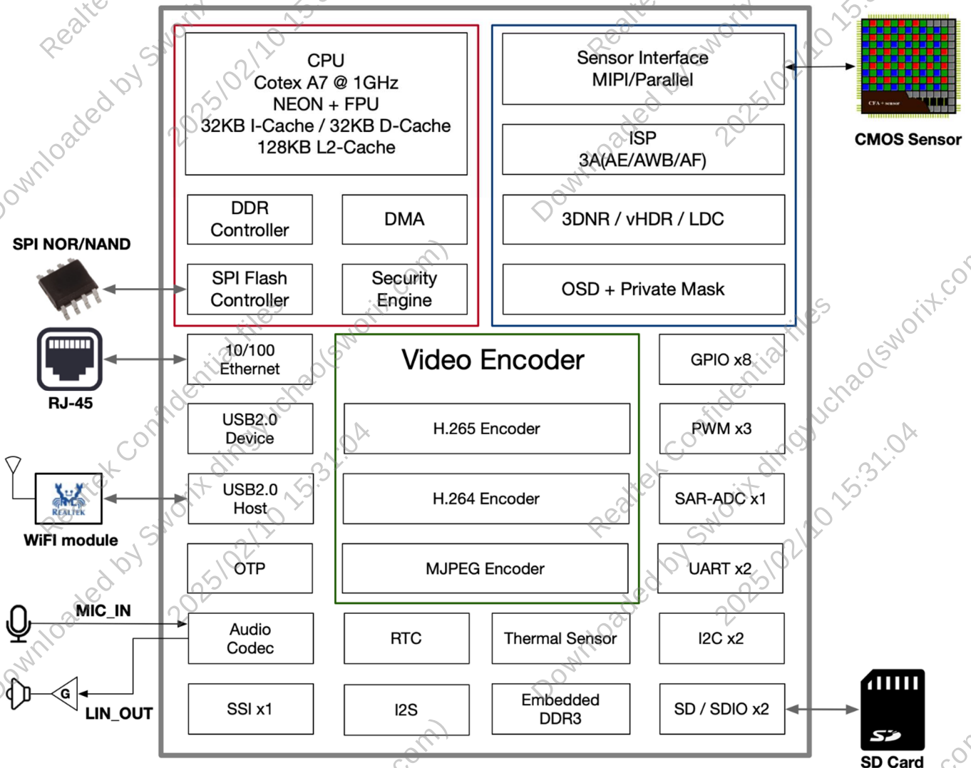
Figure 2-1 Architecture Diagram
