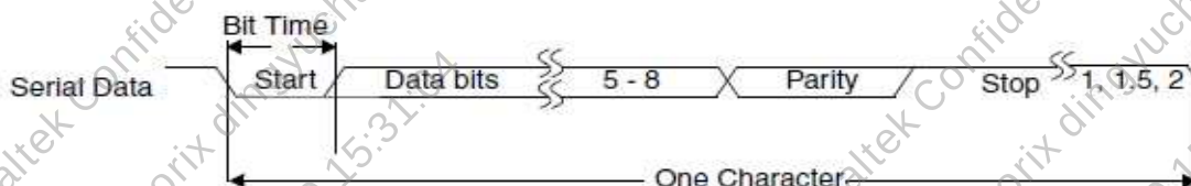
Figure 6-2 Serial Data Format
